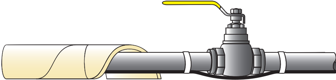
NOTE: Pipe must be wrapped with 1/2" minimum thickness fiberglass insulation
