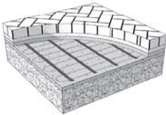
SC under Brick Pavers
