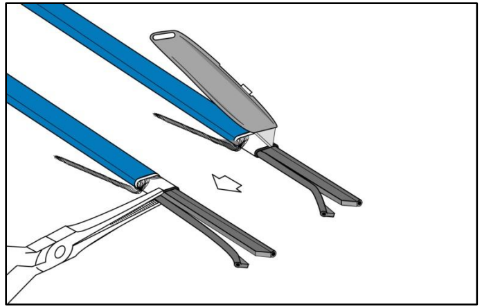
6 Score between the bus wires and bend the core to break it free and peel the core material away from the bus wires.
