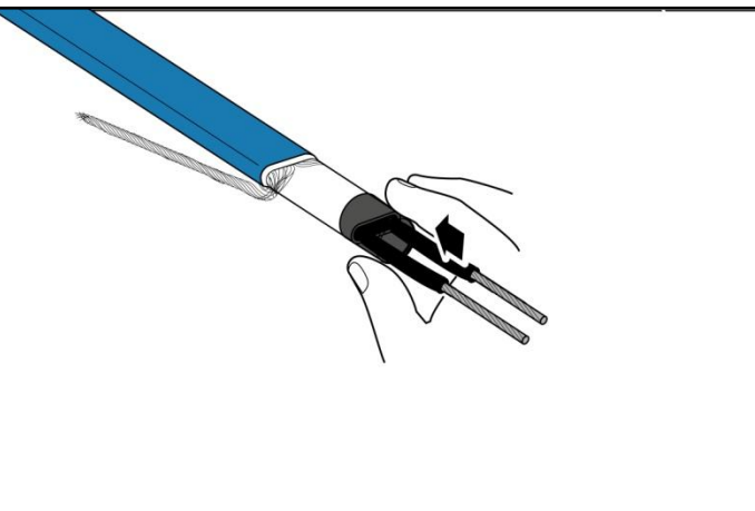
9 Center the 1/2" x 1" heat shrink tube over the cable core and bus wires as shown.
