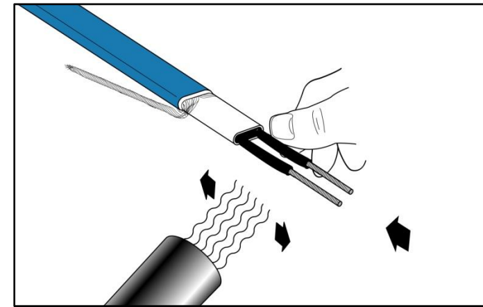
8 Slide the 1/8" dis. X 1" heat shrink tube over the bus wires. Apply heat to shrink the tubes, approximately 2 minutes at 600°F (315°C). Keep tubes up against the core while heat shrinking.
