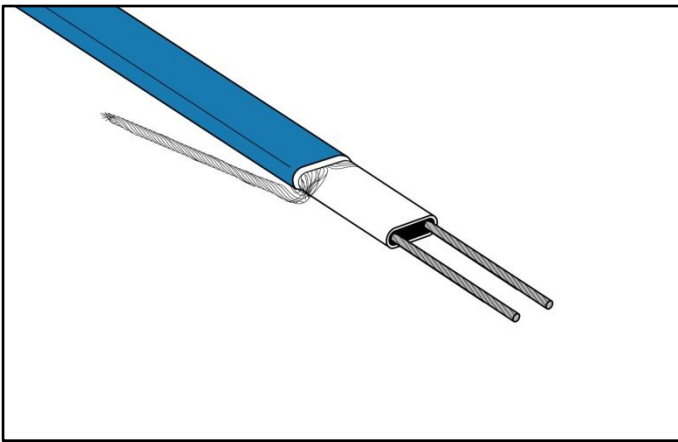
7 Cut and remove the remaining center core, leaving the bare conductors.
