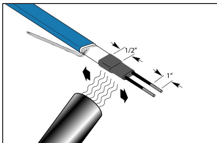
10 Heat evenly for approximately 3 minutes at 600°F (315°C) until it shrinks completely.
